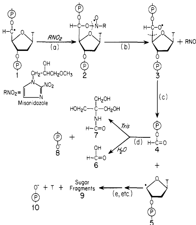
Scheme III Proposed Mechanism of Involvement of Misonidazole (RNO 2 ) in NCS-Chrom-Induced Damage at C-5'
